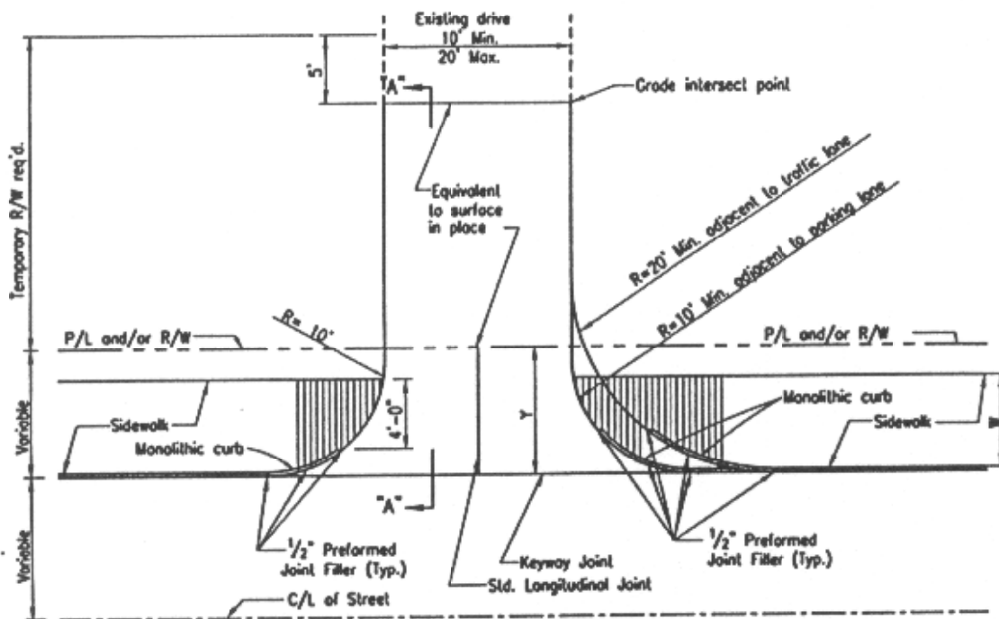
CLASS I DRIVE (PRIVATE) WITH SIDEWALK ADJACENT TO CURB Not to Scale
