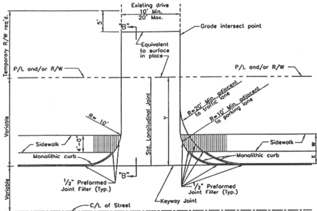
CLASS I DRIVE (PRIVATE) WITH SIDEWALK 2' TO LESS THAN 6' FROM FACE OF CURB Not to Scale
