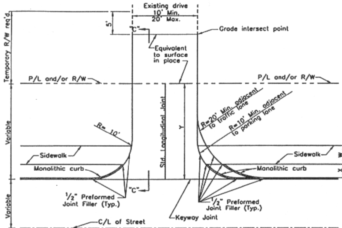
CLASS I DRIVE (PRIVATE) WITH SIDEWALK 6' AND OVER FROM FACE OF CURB Not to Scale
