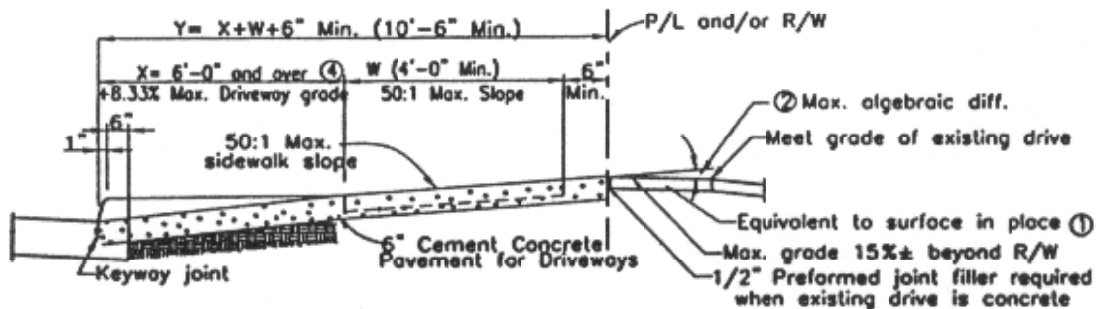
SECTION "C-C" Not to Scale
