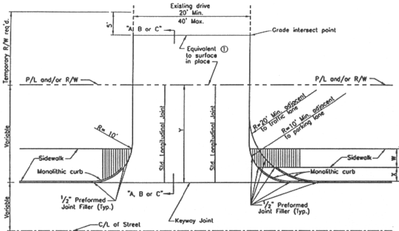
CLASS III DRIVE (COMMERCIAL) Not to Scale
